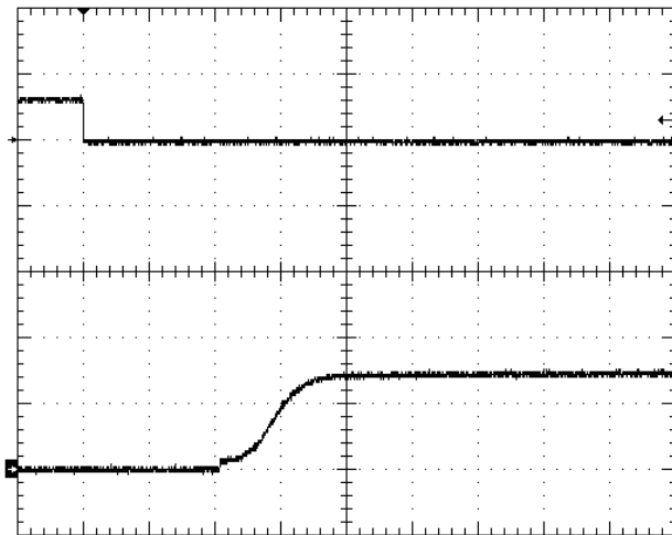
Fig.1.5V-4: Turn-on transient at full rated load current (resistive) with 10 \mu F tantalum + 1 \mu F ceramic capacitor at Vin=48V, triggered via ON/OFF pin. Top trace: ON/OFF signal (5V/div). Bottom trace: output voltage (1V/div). Time scale: 2ms/div
