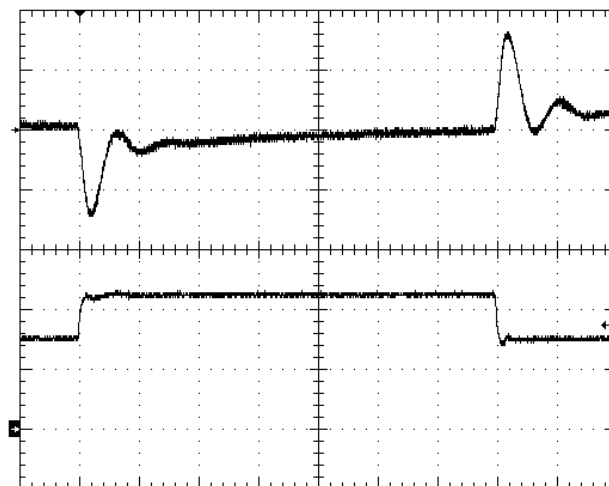
Fig.1.5V-6: Output voltage response to load current step-change (15 \Rightarrow 22.5A) at Vin=48V. Top trace: Output voltage (100mV/div). Bottom trace: load current (10A/div). Current slew rate: 5A/ \mu s. Co=470 \mu F os-con + 10 \mu F tantalum + 1 \mu F ceramic. Time scale: 100 \mu s/div
