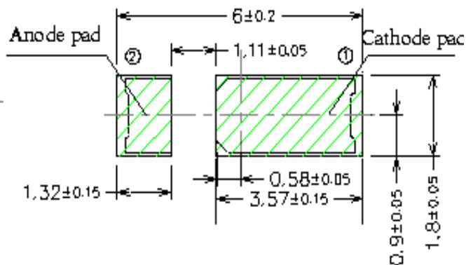
Soldering patterns
