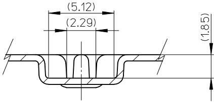
SECT. X-X
