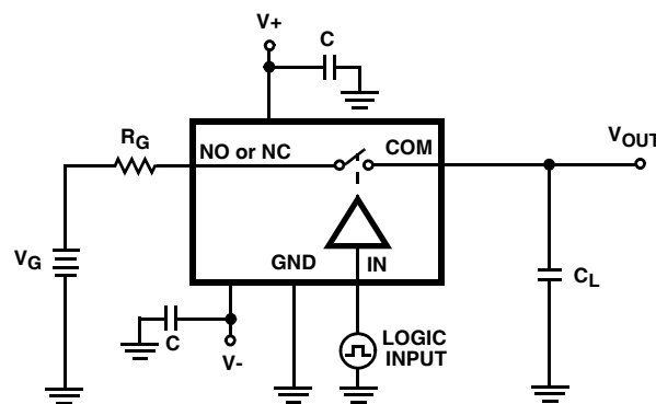
FIGURE 1. SWITCHING TIMES
