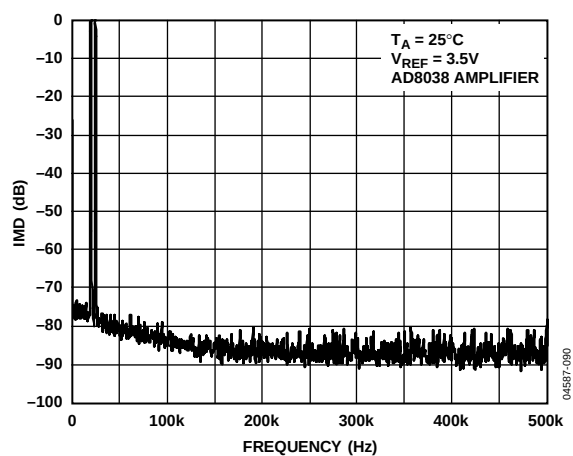
Figure 41. Wideband IMD, f_{OUT} = 20\text{ kHz} , 25 kHz, Clock = 1 MHz
