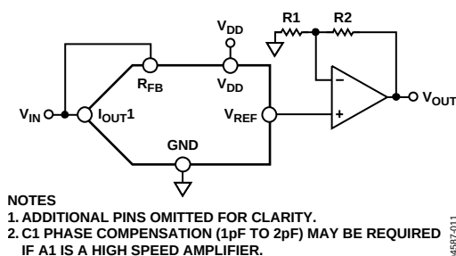
Figure 46. Single-Supply Voltage Switching Mode
