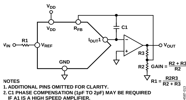
Figure 47. Increasing Gain of Current-Output DAC
