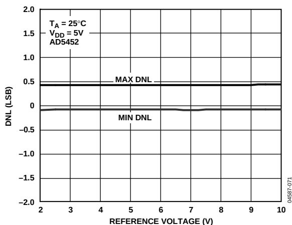
Figure 15. DNL vs. Reference Voltage
