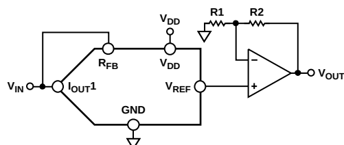
Figure 46. Single-Supply Voltage Switching Mode
