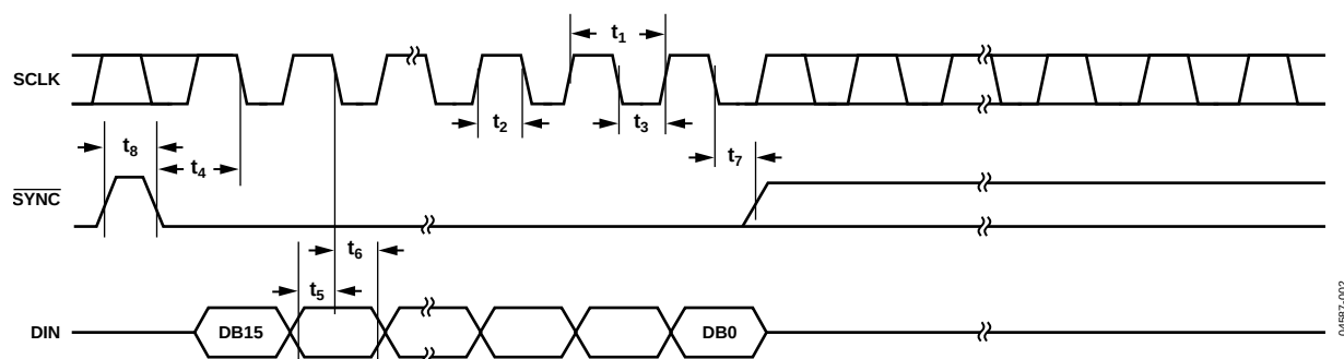
Figure 2. Timing Diagram
