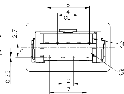
RECOMMENDED PCB LAYOUT (TOP VIEW) GENERAL TOLERANCE \pm 0.05\text{mm} (T=1.2/1.6mm)
