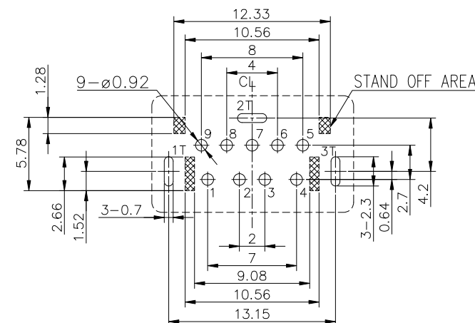
RECOMMENDED PCB LAYOUT (TOP VIEW) GENERAL TOLERANCE \pm 0.05\text{mm} (T=1.2/1.6mm)
