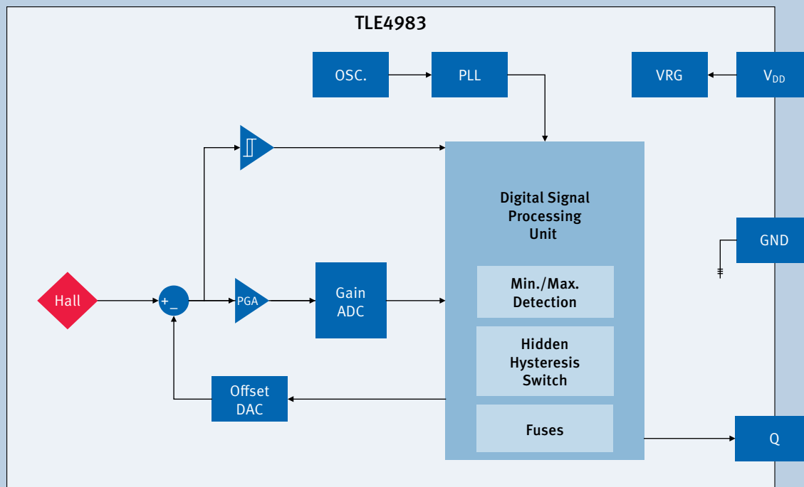
Block Diagram of TLE4983C
