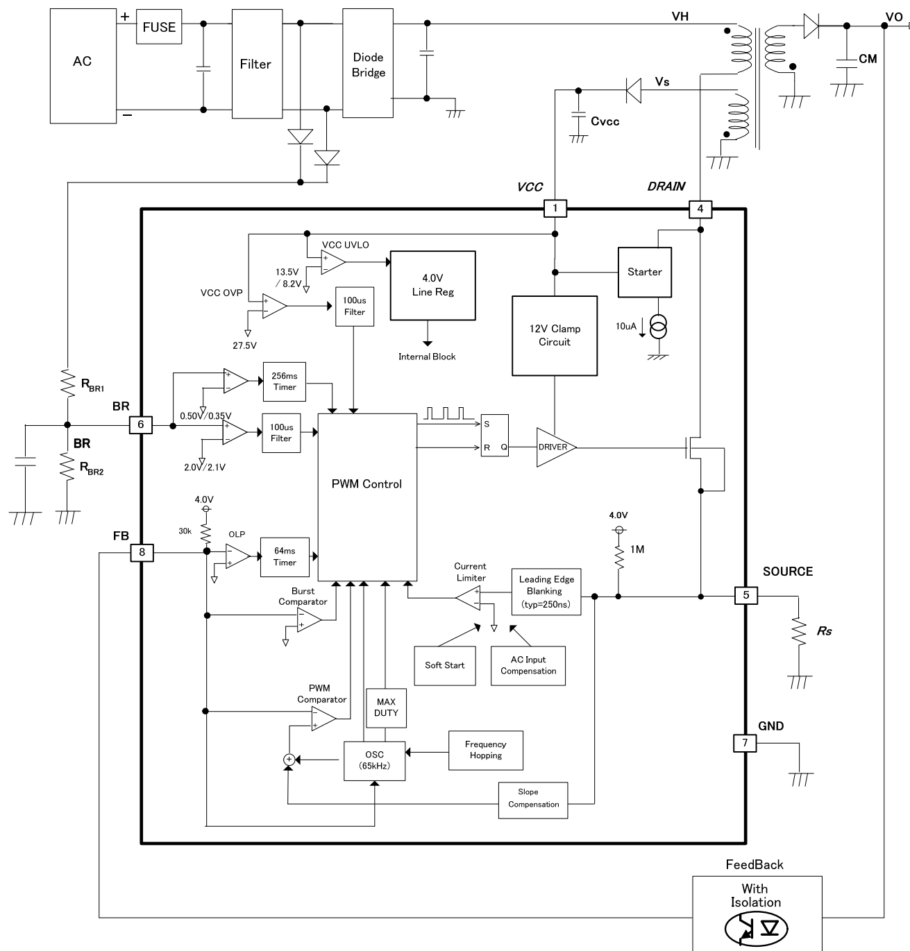
Figure 3. Block Diagram
