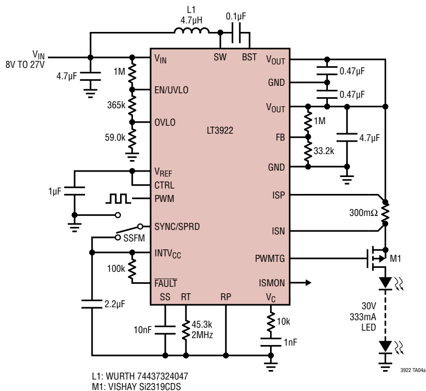
333mA Boost LED Driver Using External PWM Dimming and SSFM
