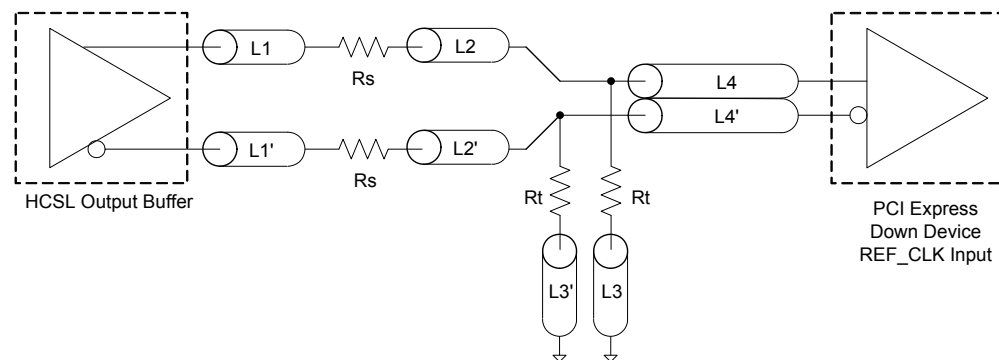
Figure 1: Down Device Routing
