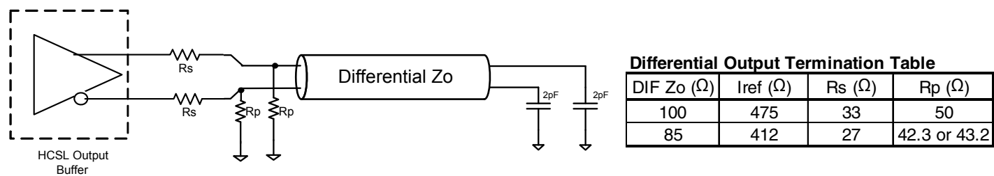
932SQ420 Differential Test Loads
