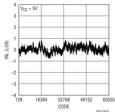
INL Curve
