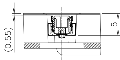
SECT. D-D (SCALE 2:1) ROTATED 90° CW
