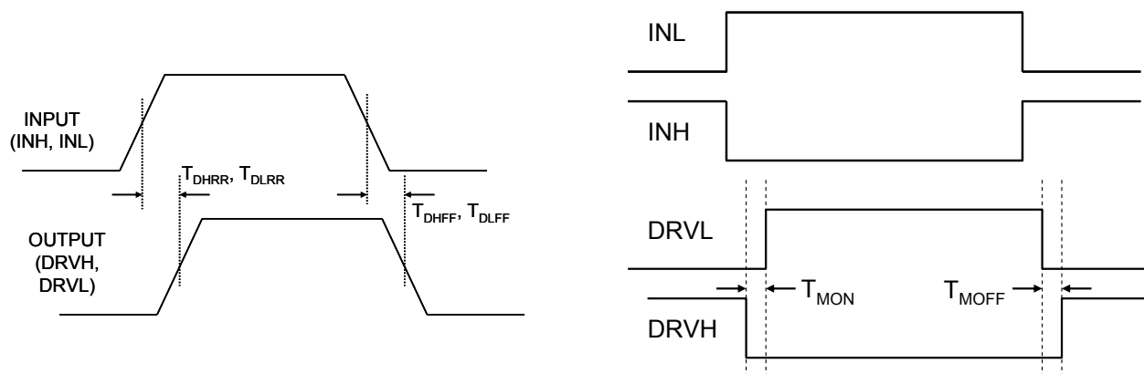
Figure 2—Timing Diagram
