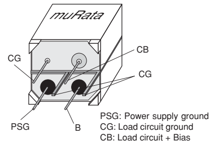
Terminal Layout (Bottom figure)
