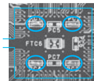
With MLCC 0.22μF×4
