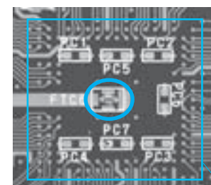
With chip 3-terminal capacitor (NFM) 1μF×1
