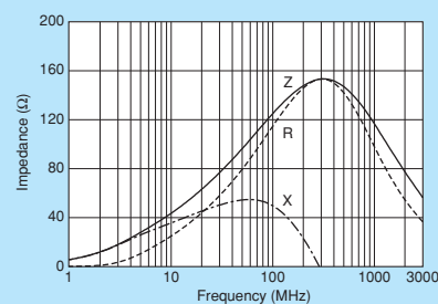
BLM31PG121SN1
