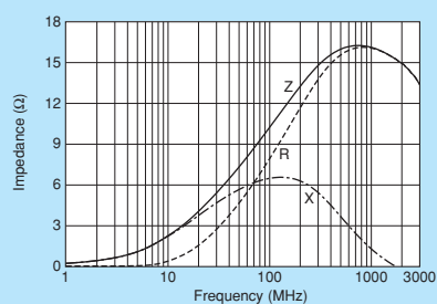
BLM15PG100SN1
