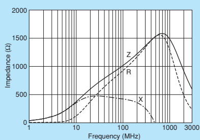
BLM15HG102SN1
