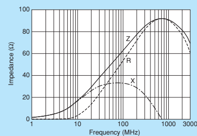
BLM15PD600SN1
