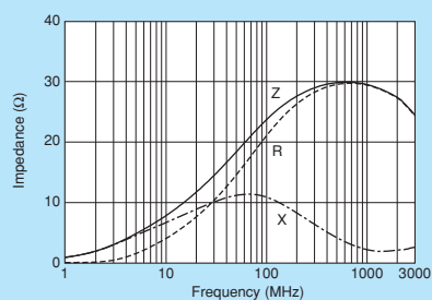
BLM21PG220SN1
