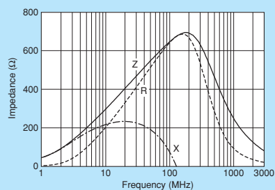
BLM18RK601SN1
