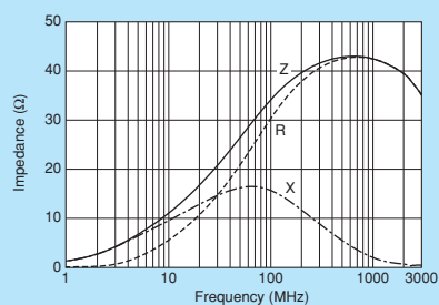
BLM21PG300SN1
