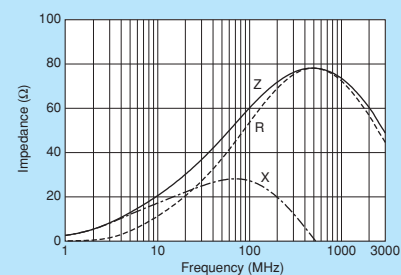
BLM21PG600SN1
