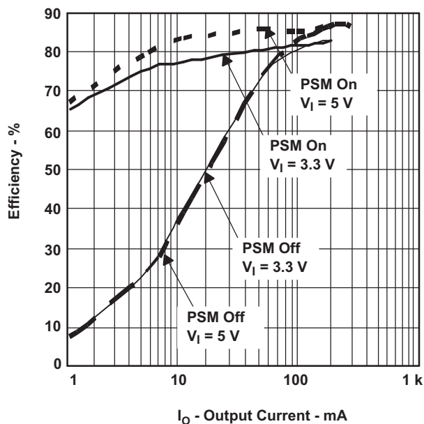
Figure 1. TPS65130 VPOS Efficiency Using the Wuerth 744031004, 4.7- \mu\text{H} Inductor
