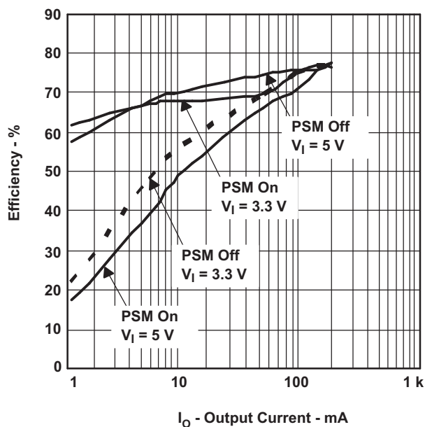
Figure 2. TPS65130 VNEG Efficiency Using Wuerth 744031004, 4.7- \mu\text{H} Inductor
