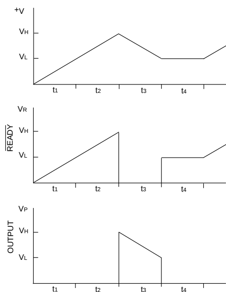
EH300/EH301 Waveforms
