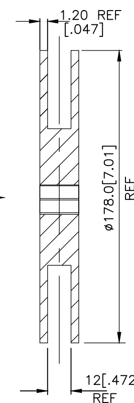
Section C—C
