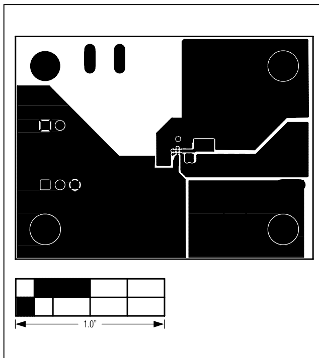
Figure 3. MAX8989 EV Kit PCB Layout—Component Side (Layer 1)
