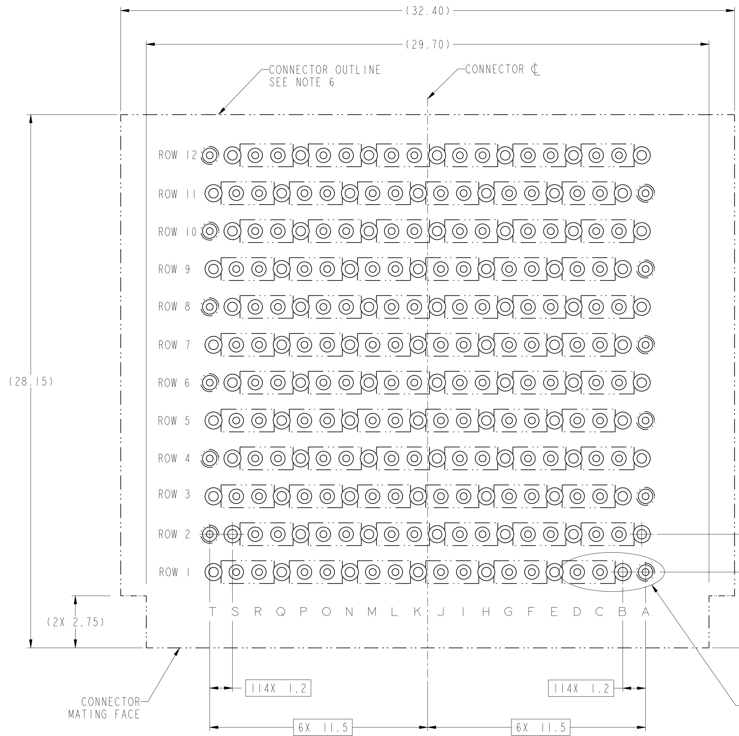
RECOMMENDED PCB LAYOUT FOR P/N 10129181-102LF AND 10129181-103LF COMPONENT SIDE NOTES 6, 7, & 9 SCALE 8:1
