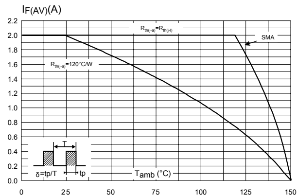
Figure 2. Average forward current versus ambient temperature ( \delta = 0.5 ) SMA
