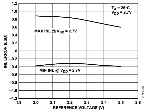
Figure 31. INL vs. V_{REF} @ V_{DD} = 2.7V
