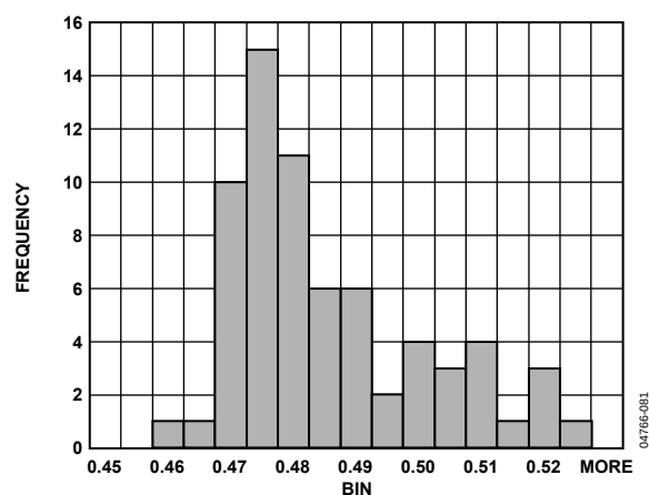
Figure 23. I_{\text{DD}} Histogram @ V_{\text{DD}} = 3\text{V}
