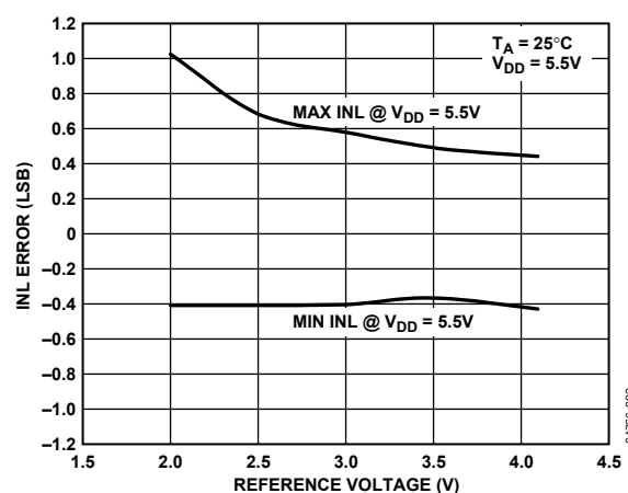
Figure 27. INL vs. V_{\text{REF}} @ V_{\text{DD}} = 5.5\text{V}
