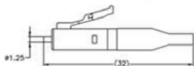
LC Simplex Behind the Wall (BTW) Connector with 900 \mu m Boot
