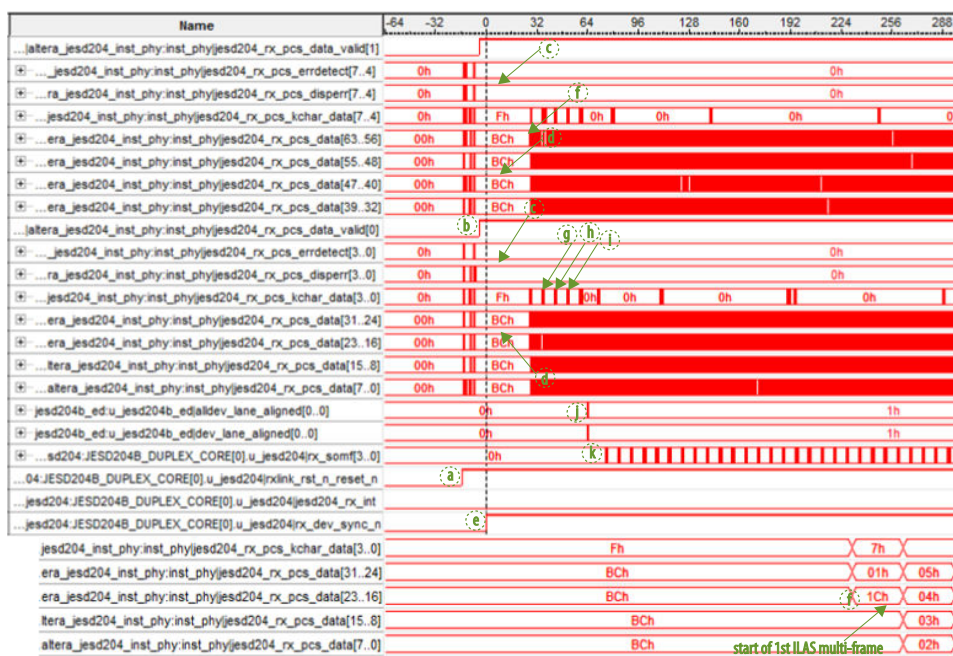
This is a Signal Tap image during the JESD204B link initialization. The JESD204B link has two transceiver channels ( L = 2 ).
