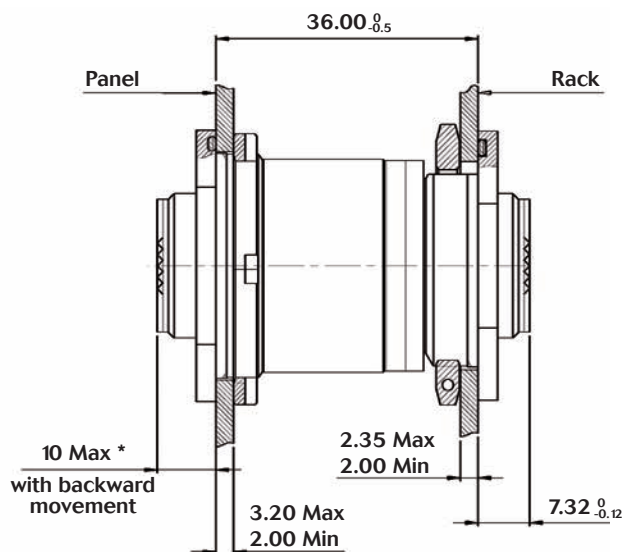
Plug type 26 & Receptacle type 27
