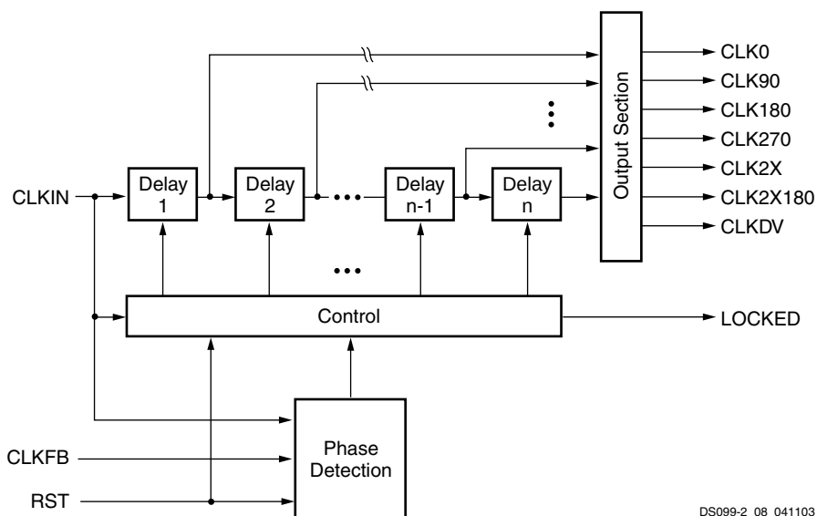
Figure 41: Simplified Functional Diagram of DLL
