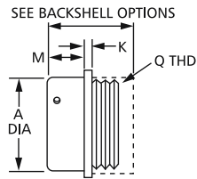
SOLDER KPT01 (MS3111)
