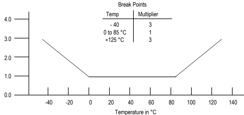
Figure 9. Temperature error multiplier (MPX5100D, MPX5100G, MPXV5100G)
