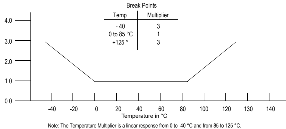
Figure 12. Temperature error multiplier (MPX5100AP)
