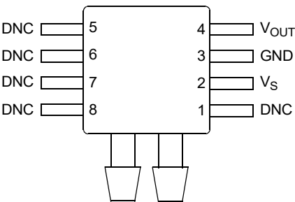
Figure 4. Device pinout (top view)
