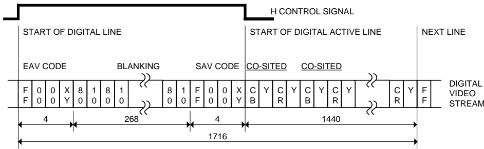
FIGURE 13. BT.656 8-BIT PARALLEL INTERFACE DATA FORMAT FOR 525/60 VIDEO SYSTEMS
