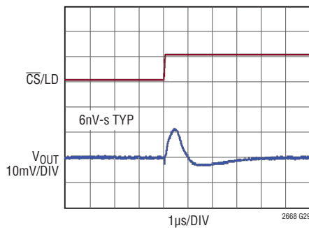
DAC-to-DAC Crosstalk
