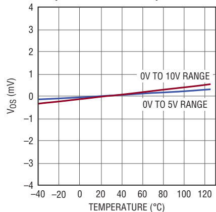
Unipolar Offset vs Temperature
