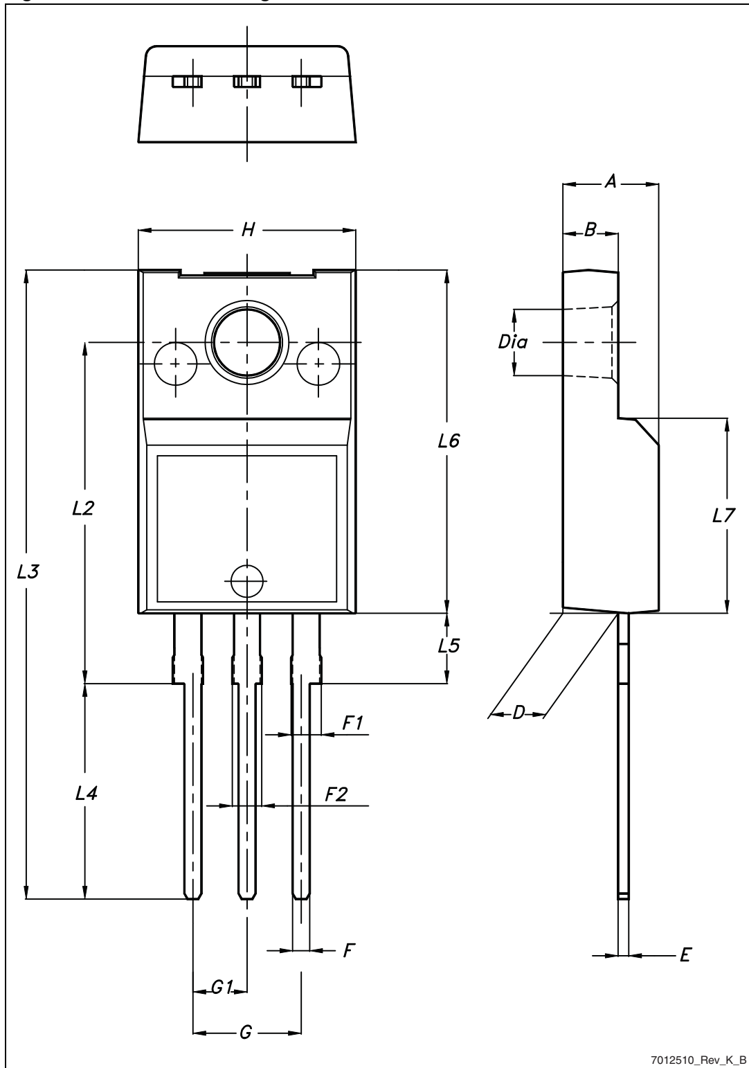
Figure 25. TO-220FP drawing
