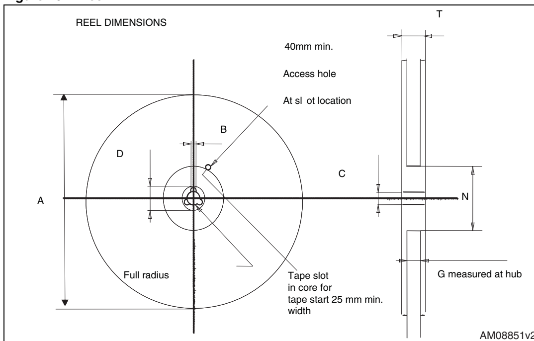
Figure 29. Reel
