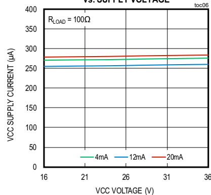
VCC SUPPLY CURRENT vs. SUPPLY VOLTAGE
