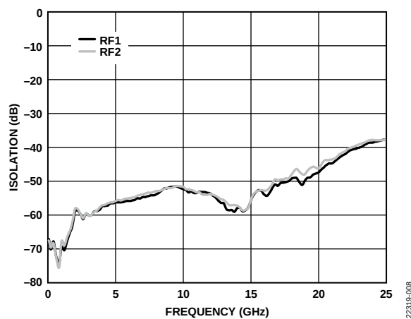
Figure 8. Isolation vs. Frequency, Between RFC and RF1/RF2
