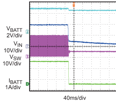
Power Off Waveform
