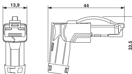
RJ45 connector, IP20, angled
