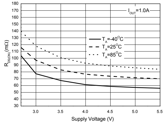
Figure 7. R DS(ON) vs. Supply Voltage
