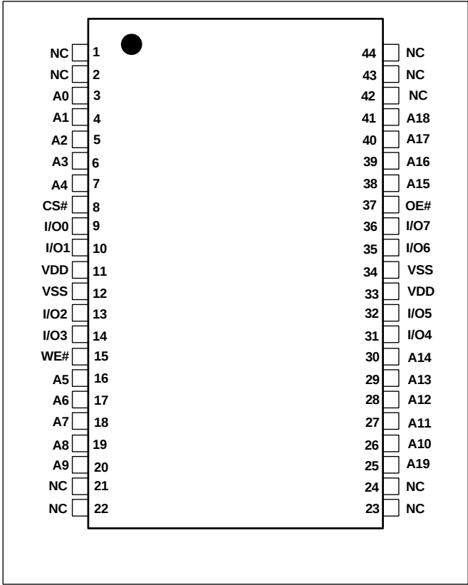
44-Pin TSOP-II
