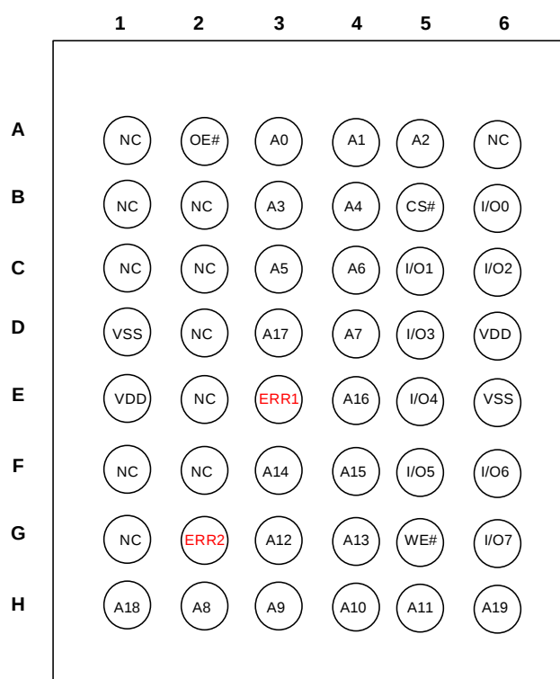
48-Pin mini BGA (6mm x 8mm), ERR1/2
