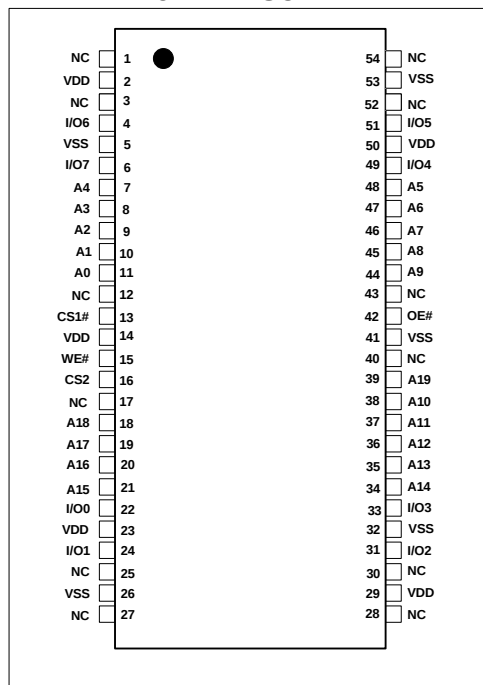
54-Pin TSOP-II
