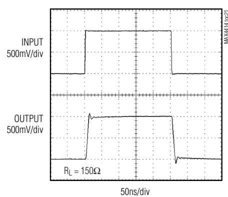
MAX4414/MAX4416/MAX4418 LARGE-SIGNAL PULSE RESPONSE
