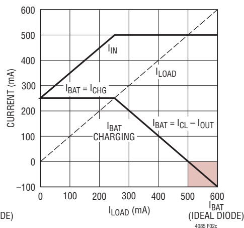
(2c) High Power Mode with I_{CL} = 500mA and I_{CHG} = 250mA R_{PROG} = 100k and R_{CLPROG} = 2k
