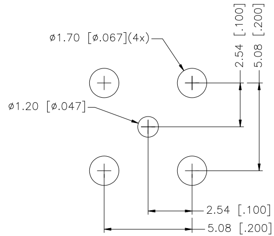
PCB MOUNTING HOLES
