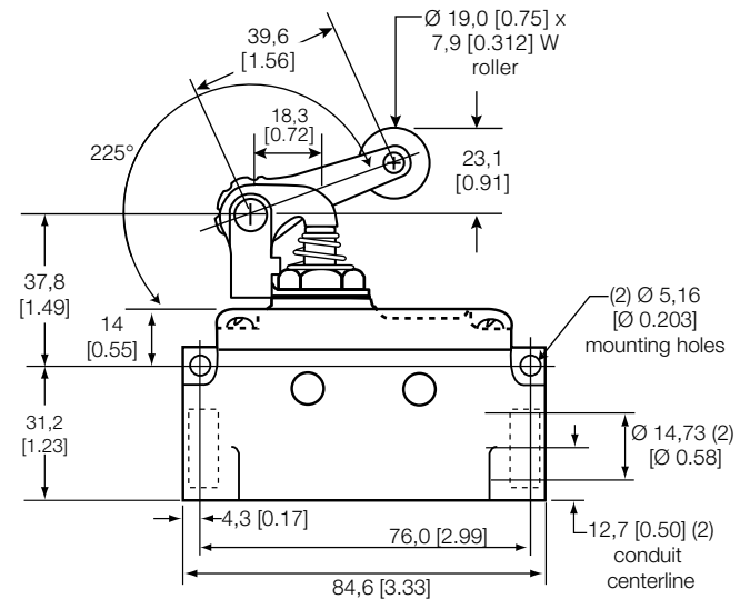
Figure 25. E9 Series, roller lever, side mount
