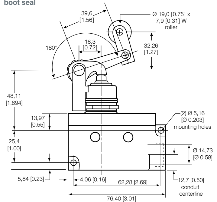
Figure 4. E7 Series, one-way roller lever, diagonal mount with boot seal
