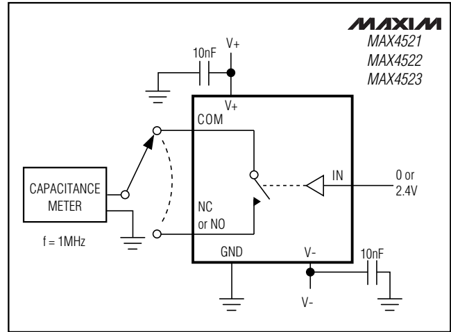
Figure 6. Channel Off-Capacitance
