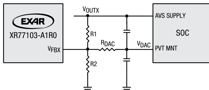
Figure 29. AVS Control
