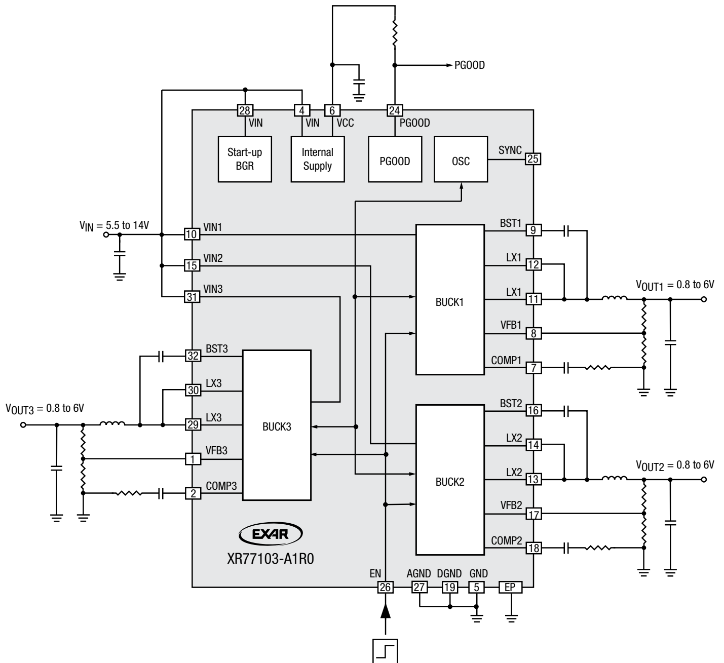
Figure 1. Typical Application
