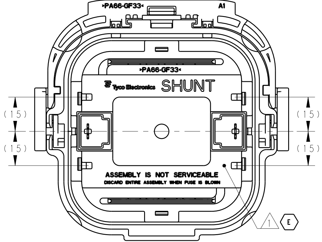
1-2103212-7 & 2-2103212-7 SHUNT
